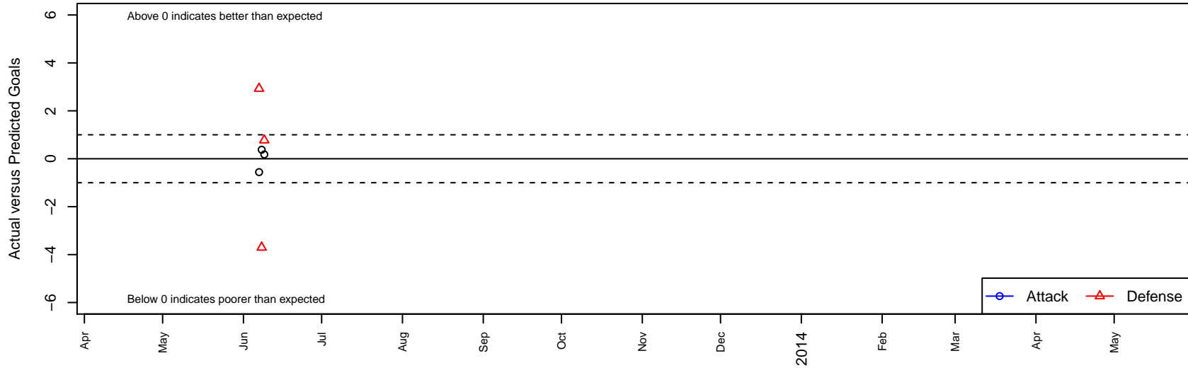
Juneau Taku Blast B01 Dots are actual minus expected GF (blue circles) and GA (red triangles). Blue line is smoothed change in attack strength. Red is smoothed change in defense strength.
